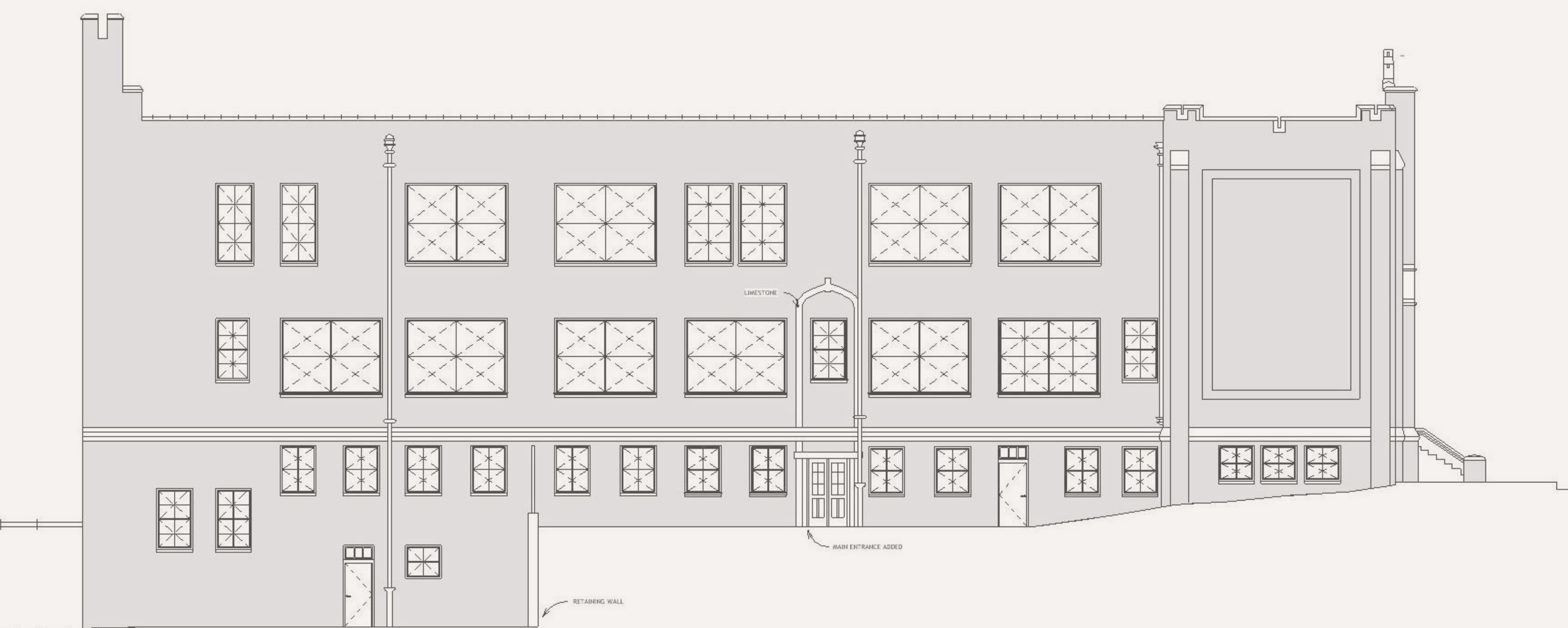
East Elevation
