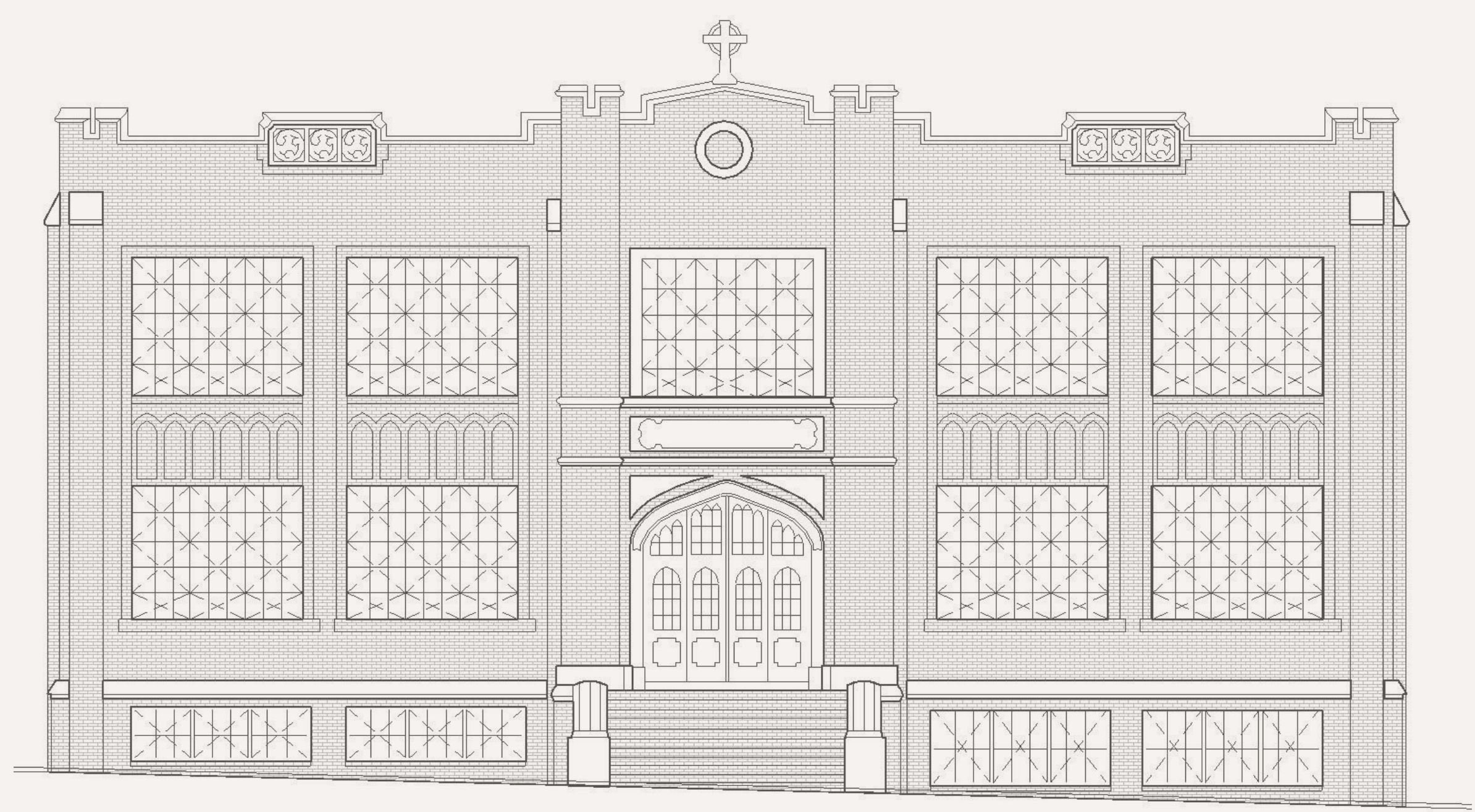
North Elevation
