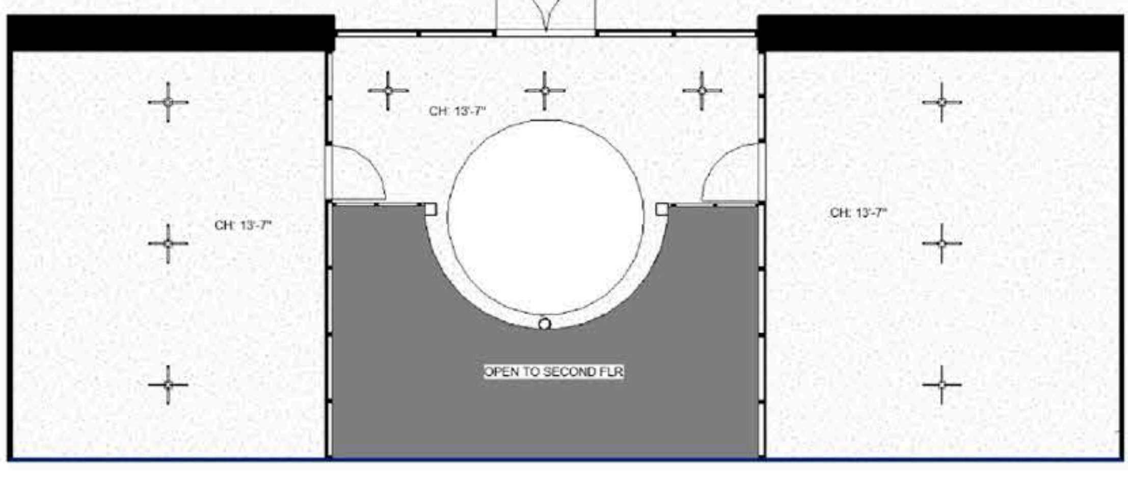
Enlarged Atrium Ceiling Plan
