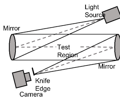
Schlieren Imaging Setup
